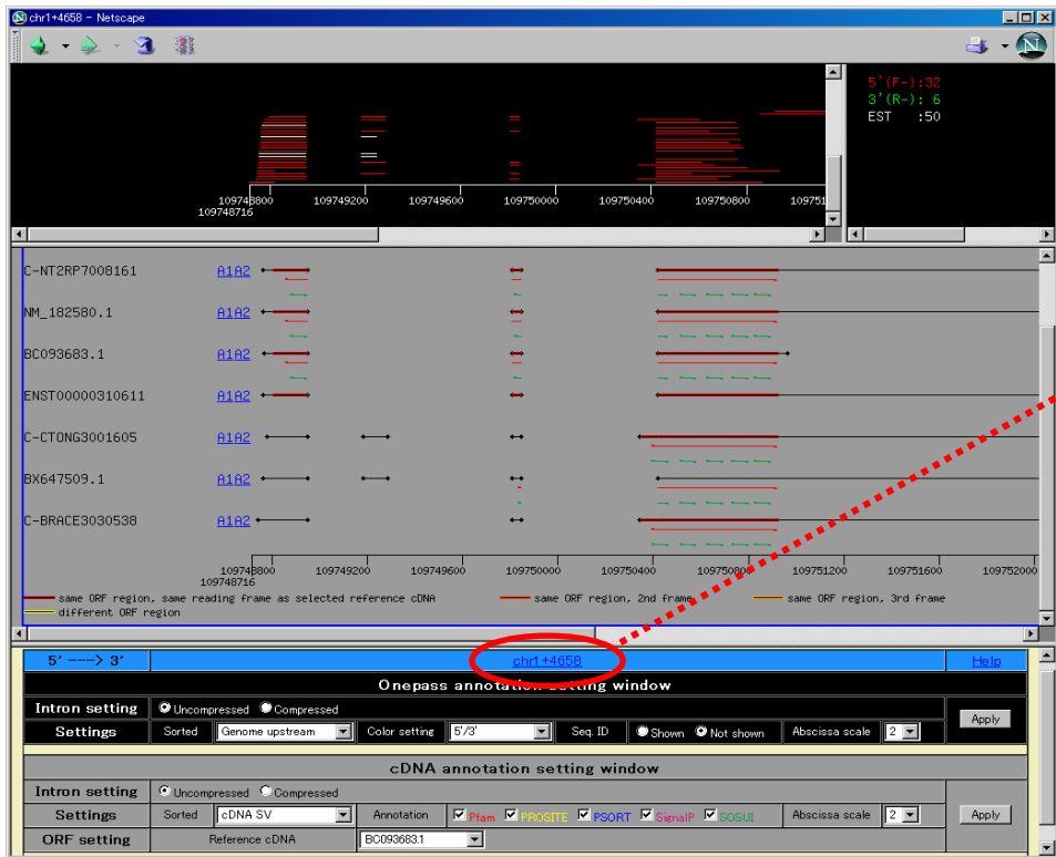
Fig2-11 Annotation and genome mapping viewer (mRNA variation viewer)
